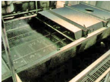
Easy Maintenance with Segmented Screen Decks and Top Cover
